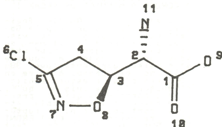
Acivicin
